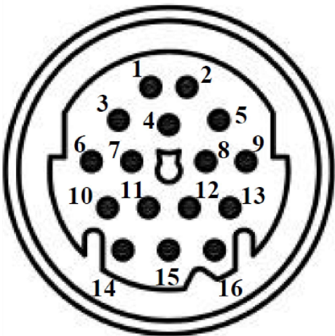
Transmission Solenoid Connector Harness Connector Pin View
