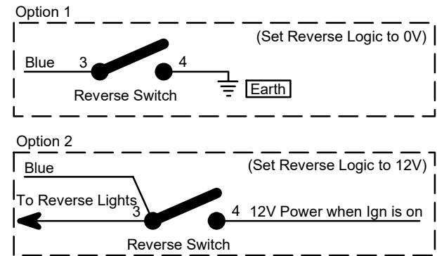
Transmission Selector Switch
