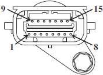
NB! Gearbox Conector Pin View
