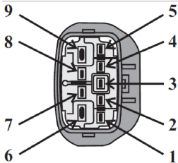
NB! Gearbox Plug Pin View
