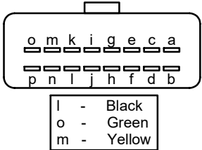
Receiver Connector pin view
