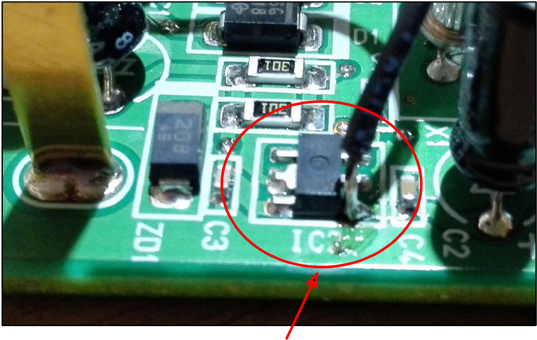
Connect Red wire to Regulator
