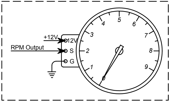
Digital Tachometer Wiring
