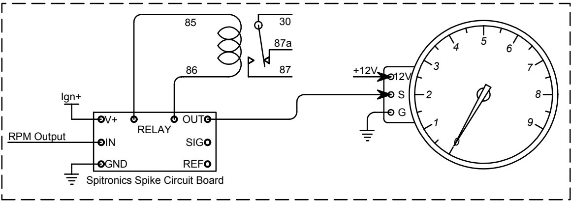
High Voltage Spike Tachometer Wiring
