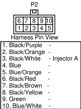
Connector Pinouts
