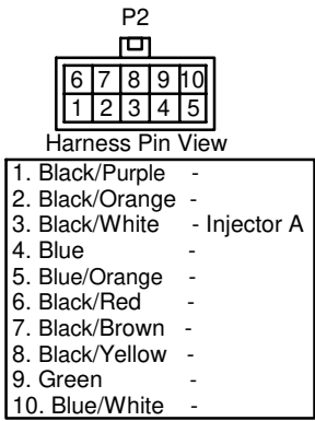
Connector Pinouts
