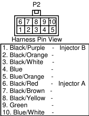
Connector Pinouts
