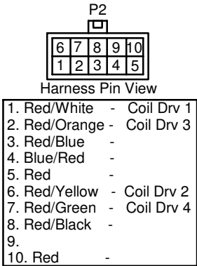
Connector Pinouts
