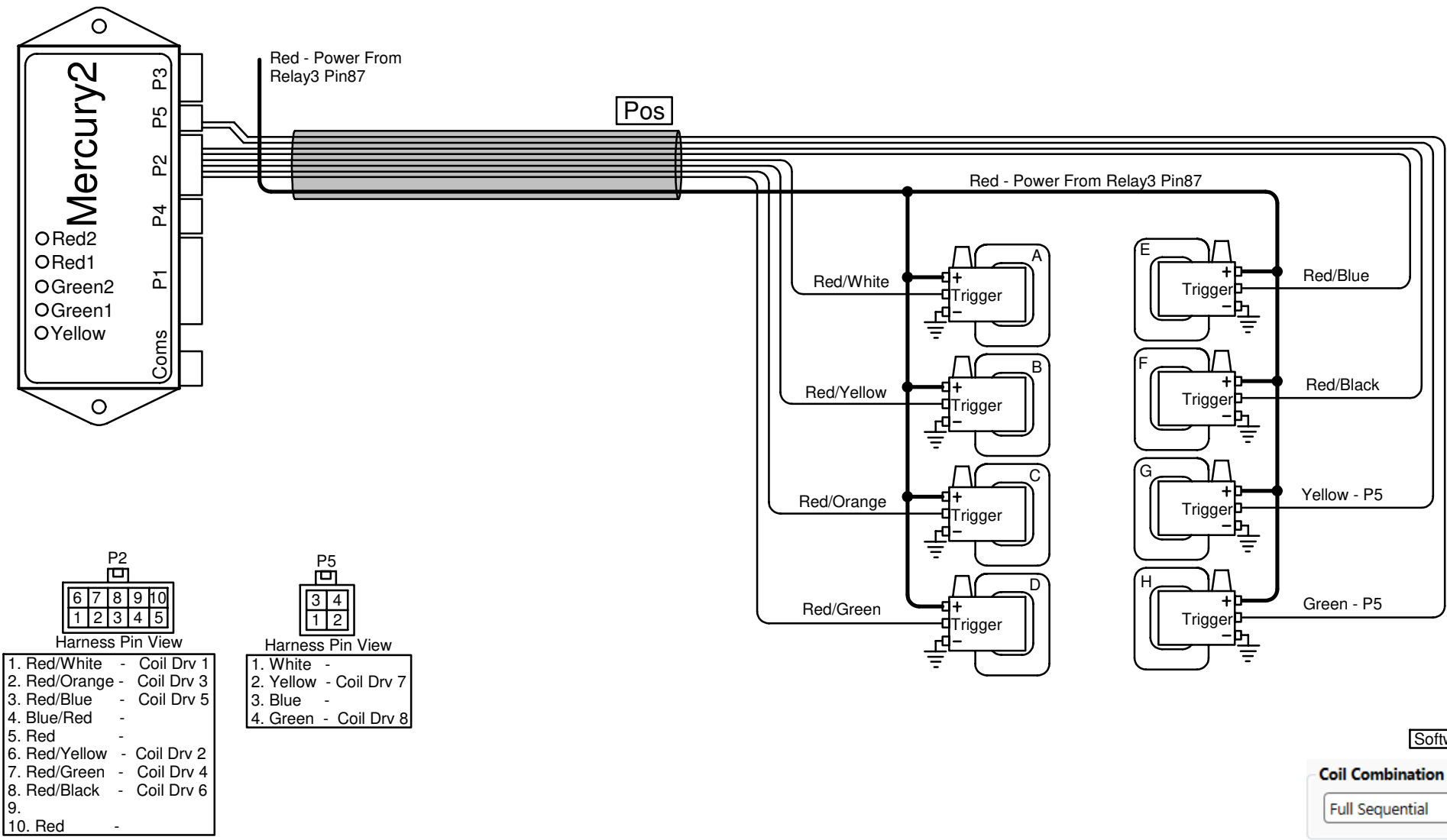
Connector Pinouts
