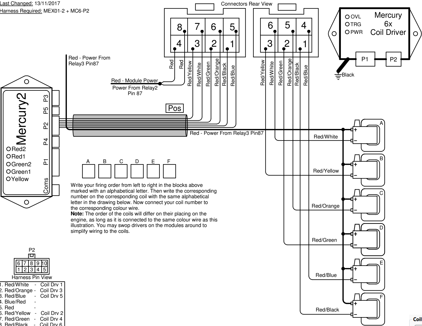
Connector Pinouts
