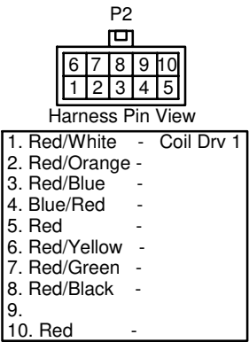
Connector Pinouts
