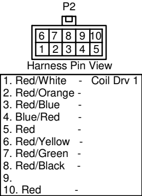
Connector Pinouts
