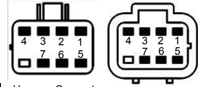
Harness Connector Pin View
